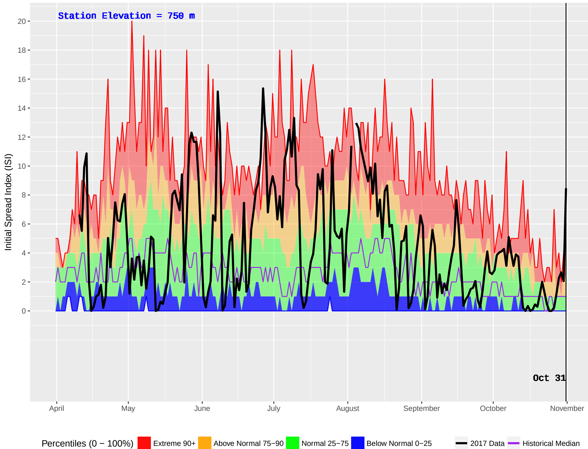
FORT ST JAMES (146) : Historical (1979–2016) and Current (2017) Noon Initial Spread Index (ISI)
