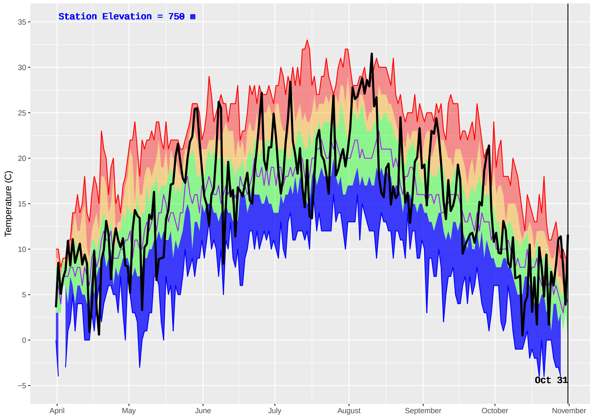
FORT ST JAMES (146) : Historical (1979–2016) and Current (2017) Noon Temperature
