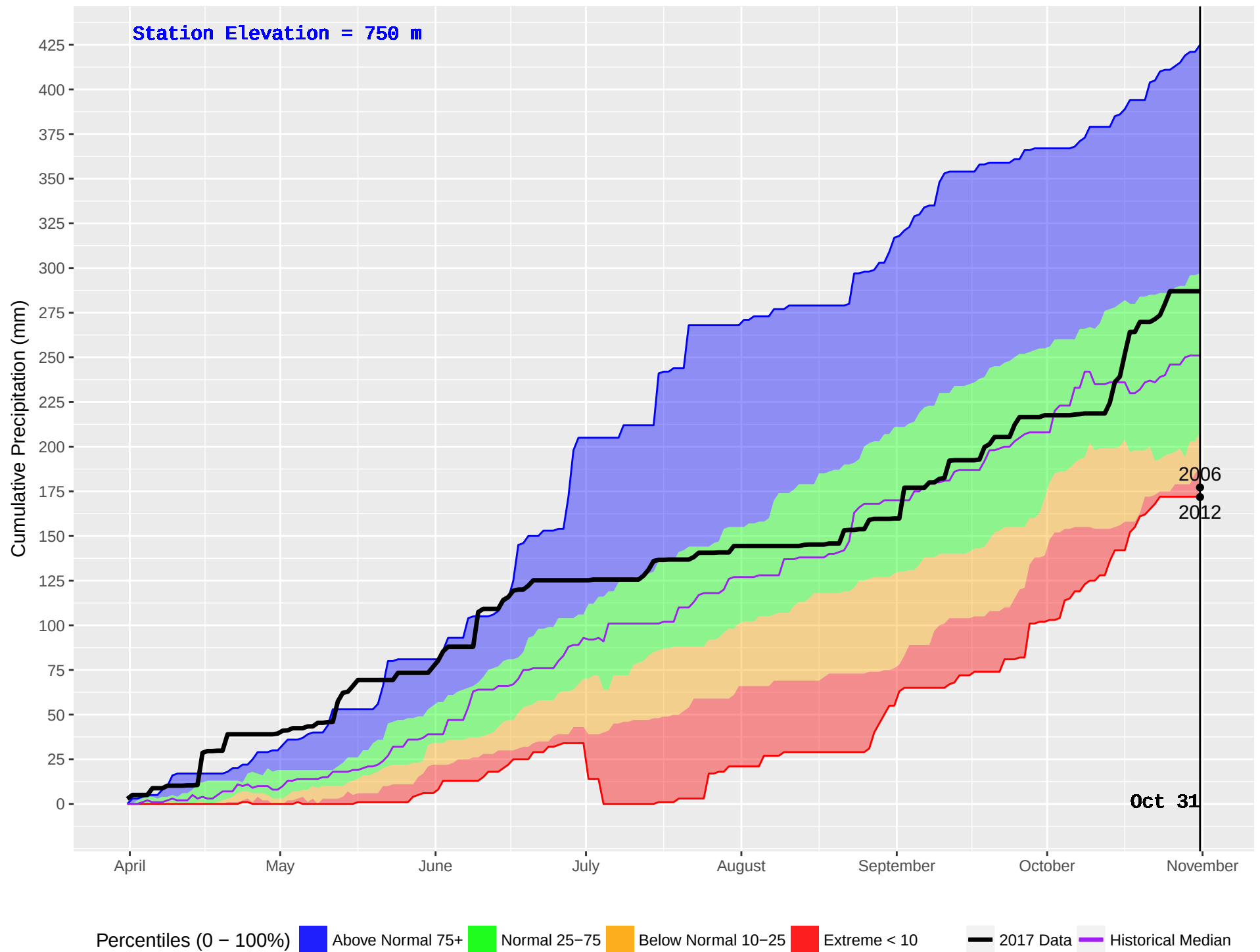
FORT ST JAMES (146) : Historical (1979–2016) and Current (2017) Noon Cumulative Precipitation
