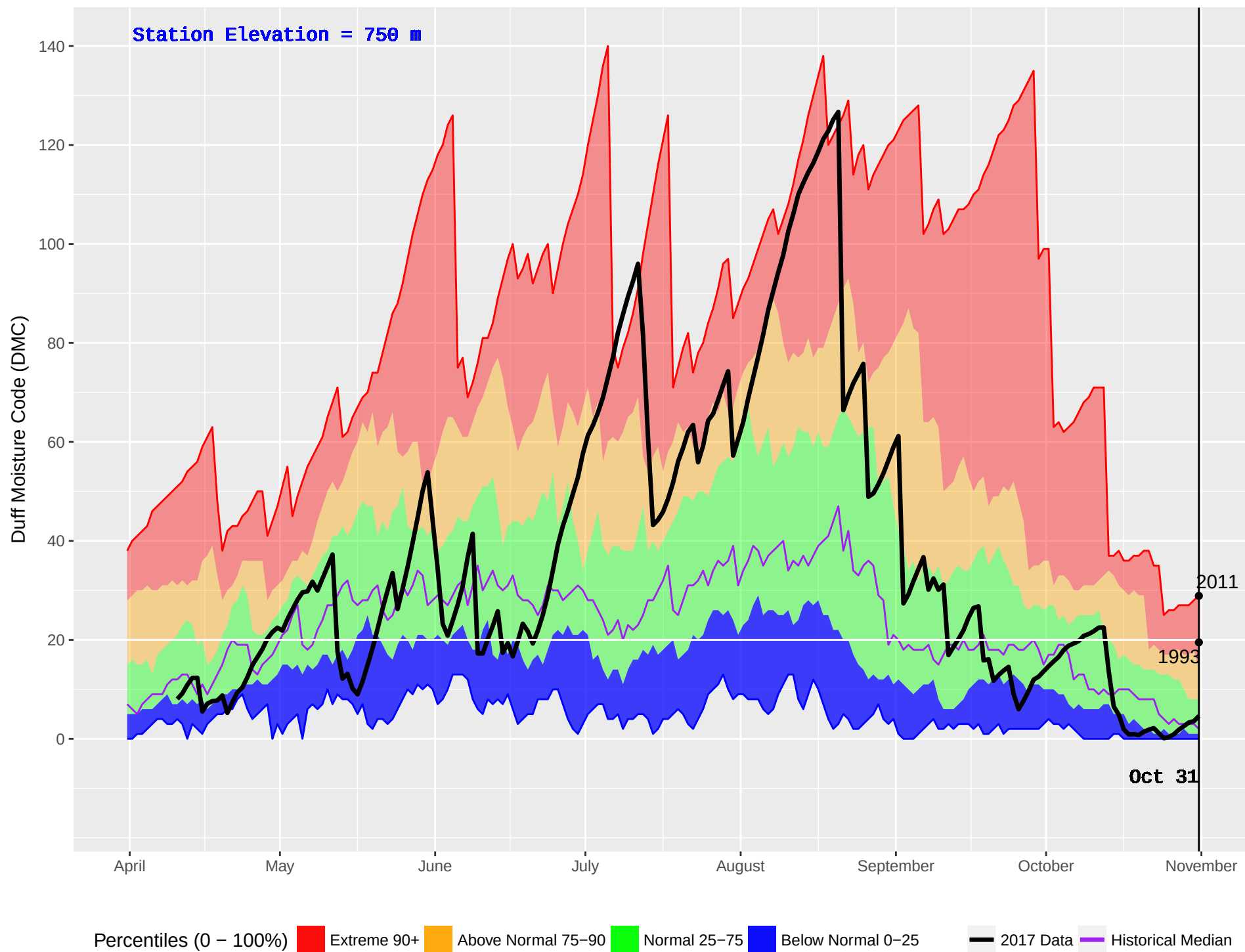
FORT ST JAMES (146) : Historical (1979–2016) and Current (2017) Noon Duff Moisture Code (DMC)
