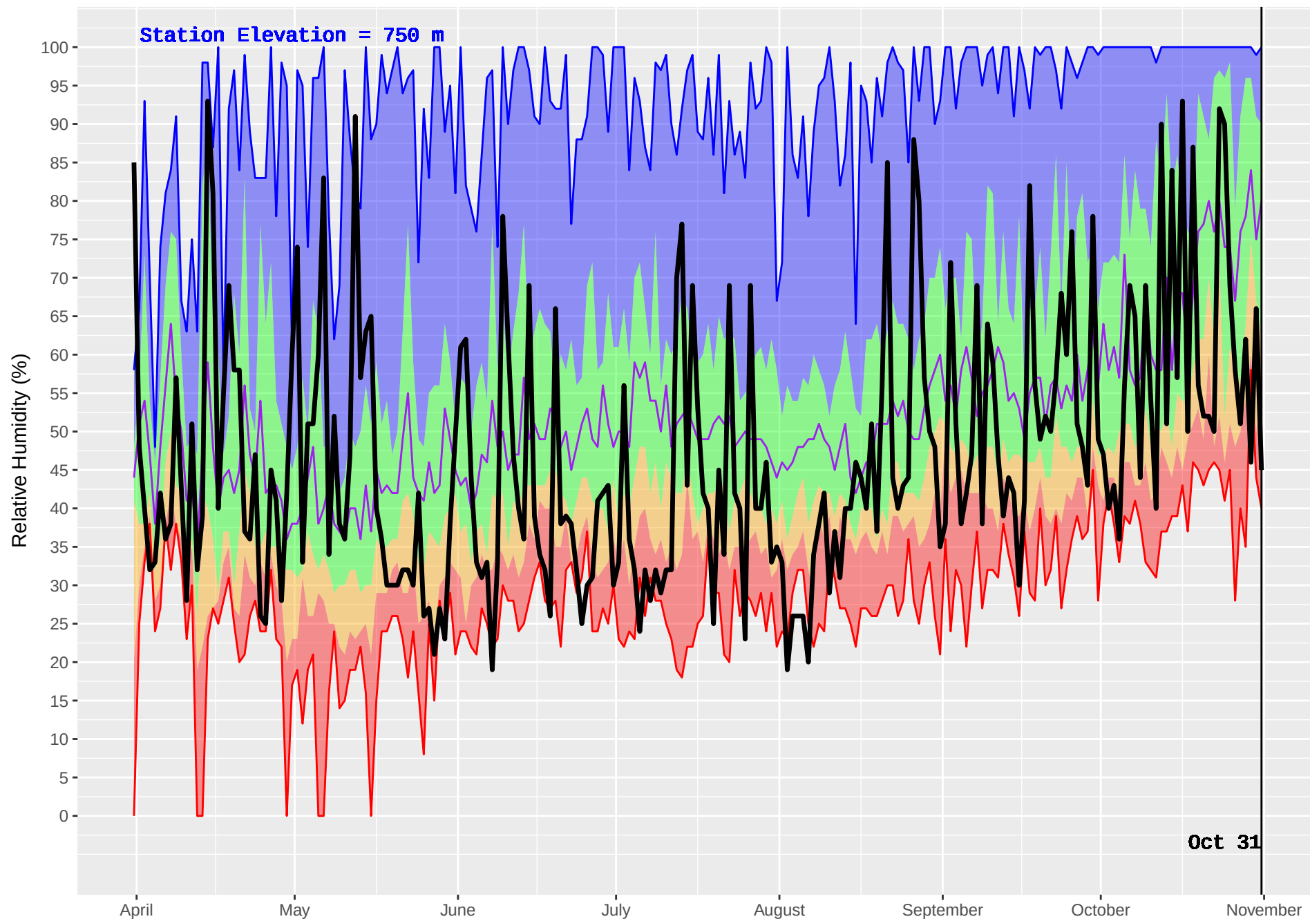
FORT ST JAMES (146) : Historical (1979–2016) and Current (2017) Noon Relative Humidity
