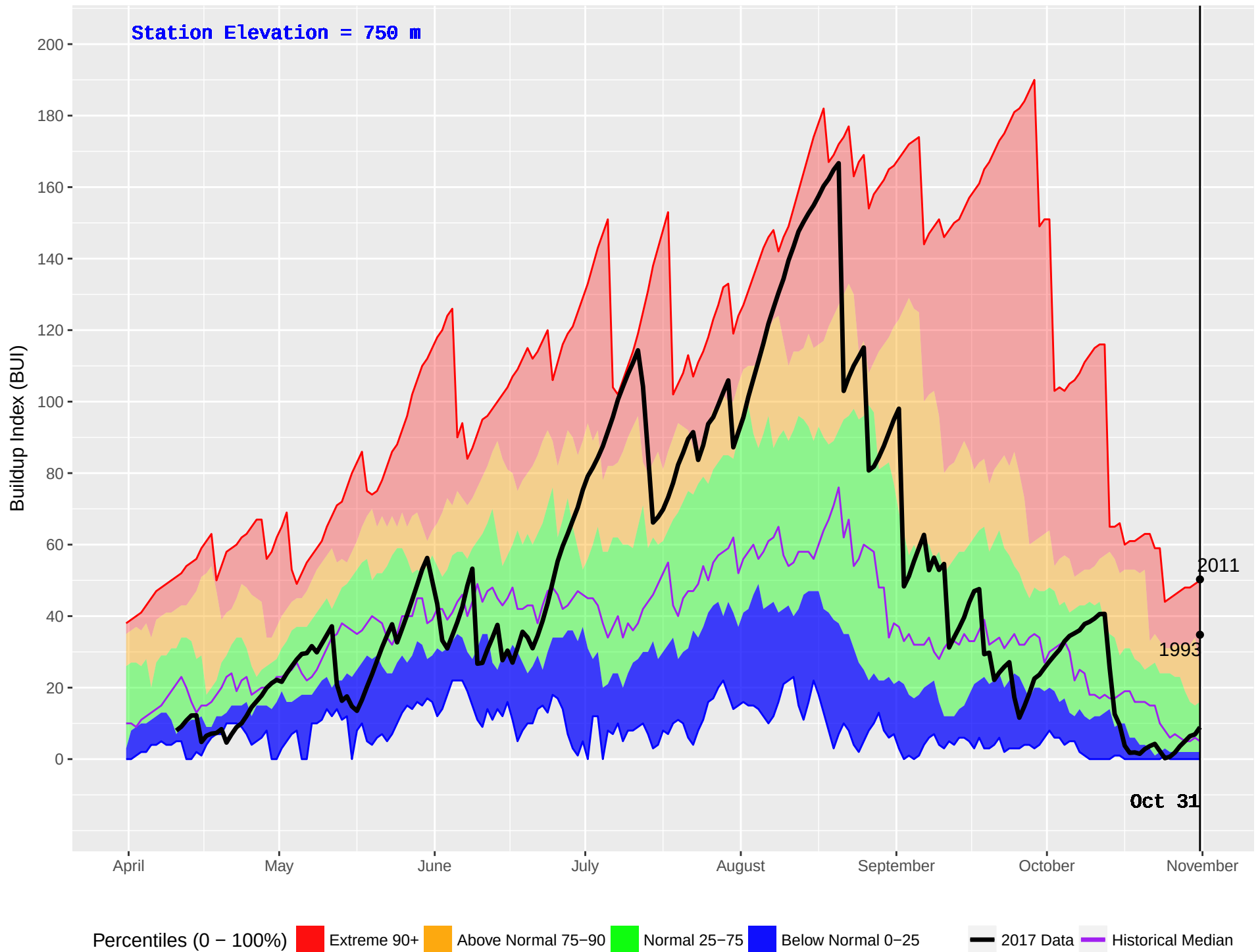
FORT ST JAMES (146) : Historical (1979–2016) and Current (2017) Noon Buildup Index (BUI)
